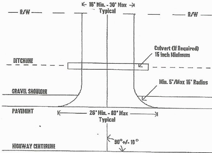
PLAN VIEW (Non-Commercial Typical)
