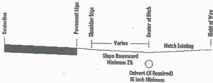
PROFILE VIEW (Typical)
